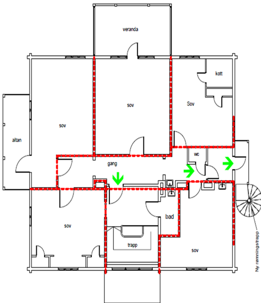
Brannplan 02 1 : 100
