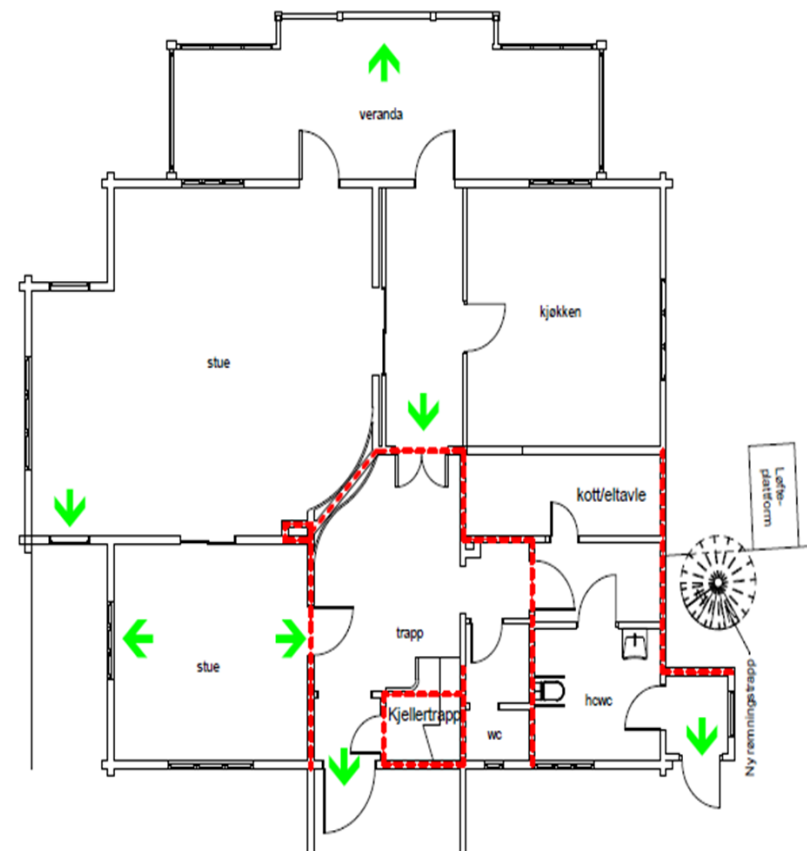
Brannplan 01 1 : 100
